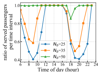
Fig. 13: Impact of Extra Vehicles
