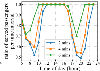
Fig. 16: Impact of detour constraint
