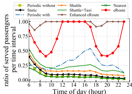
Fig. 10: Solutions' performance in unit time over a day
