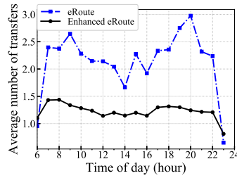
Fig. 19: Overhead of eRoute
