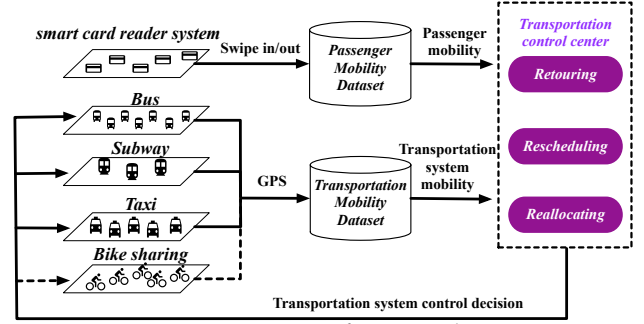
Fig. 2: eRoute framework
