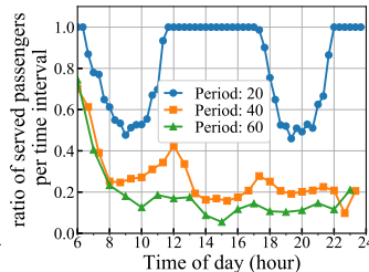
Fig. 15: Impact of Update Period
