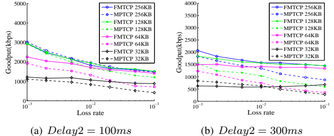
Fig. 8: The total goodput of FMTCP and MPTCP under various buffer limitations. The parameters of the subflow 1 remain the same (100ms delay, 0.1% packet loss). The delay of the subflow 2 is set to 100ms/300ms and the loss rate is between 0.1% and 10%.
