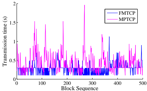
Fig. 13: The delivery delay of blocks of FMTCP and IETF-MPTCP. The parameters of subflow 1 remain the same (100ms delay, no packet loss). The delay of subflows 2 is 100ms while the loss rate is 10%.
