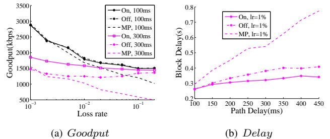
Fig. 14: The Goodput gain and delay reduction of rateless coding and scheduling in FMTCP. The buffer size is set to 128KB. The parameters of subflow 1 remain the same (100ms delay, 0.1% packet loss). The loss rate and delay of subflow 2 change according to the legend.
