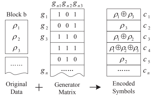
Fig. 4: Rateless Coding
