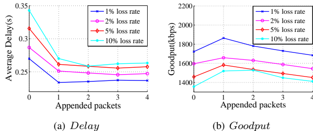
Fig. 7: Average delivery delay and goodput under different appending rate settings. The parameters of the subflow 1 remain the same (100ms delay, 0.1% packet loss). The path delay of subflow 2 is 100ms while the loss rate changes according to the legend.
