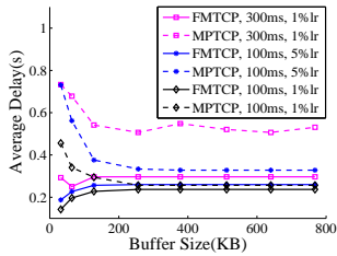
Fig. 9: The average delay of FMTCP and MPTCP under various buffer limitations. The parameters of the subflow 1 remain the same (100ms delay, 0.1% packet loss). The delay and loss rate of the subflow 2 changes according to the legend.
