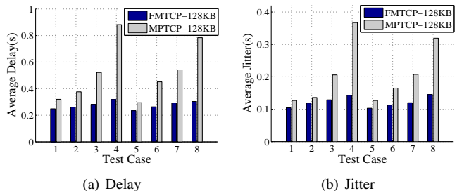
Fig. 12: The average delivery delay and jitter of blocks of FMTCP and IETF-MPTCP. The parameters of the subflow 1 remain the same (100ms delay, 0.1% packet loss). The delay and loss rate of the subflow 2 are shown in Table II.
