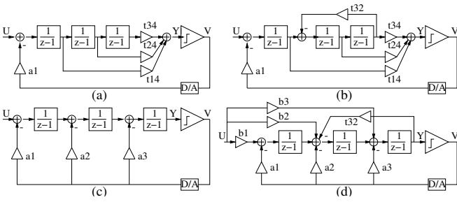
Figure 1: 3^{rd} order \Delta\Sigma modulator topologies
