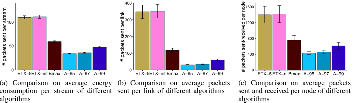
Fig. 9: Energy consumption comparison in different aspects between ETX-based, Bmax-based, and our algorithm
